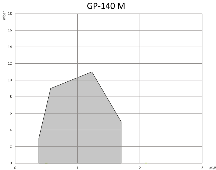
Working diagram GP-140 M LN80 ver. 1
