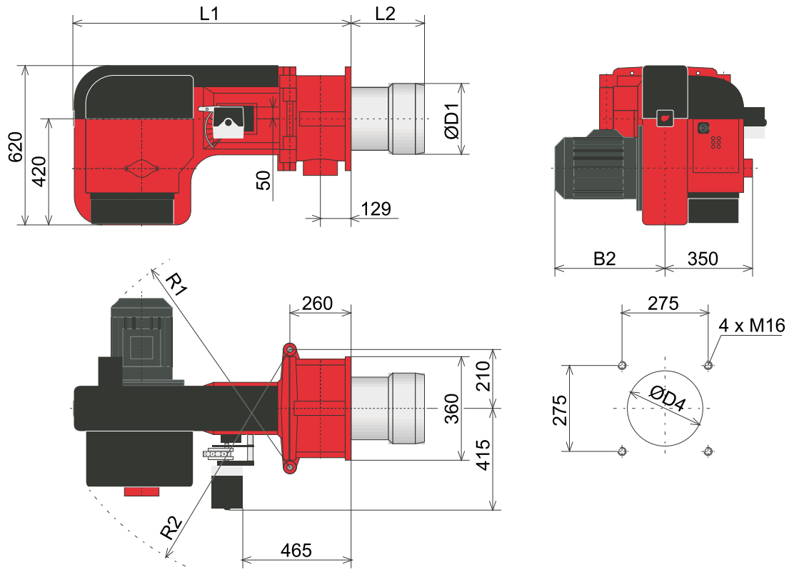
Burner measurements ver. 1
